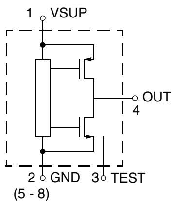
Fig. 4–5: Pin configuration
